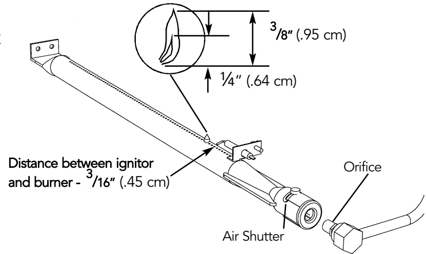
Fig. 2 SMOKER BURNER (If applicable)
