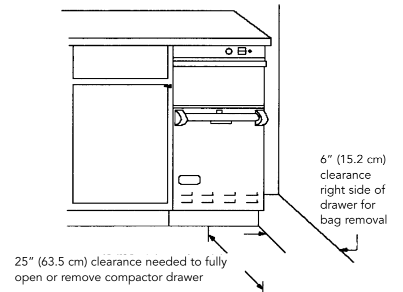
CLEARANCES
